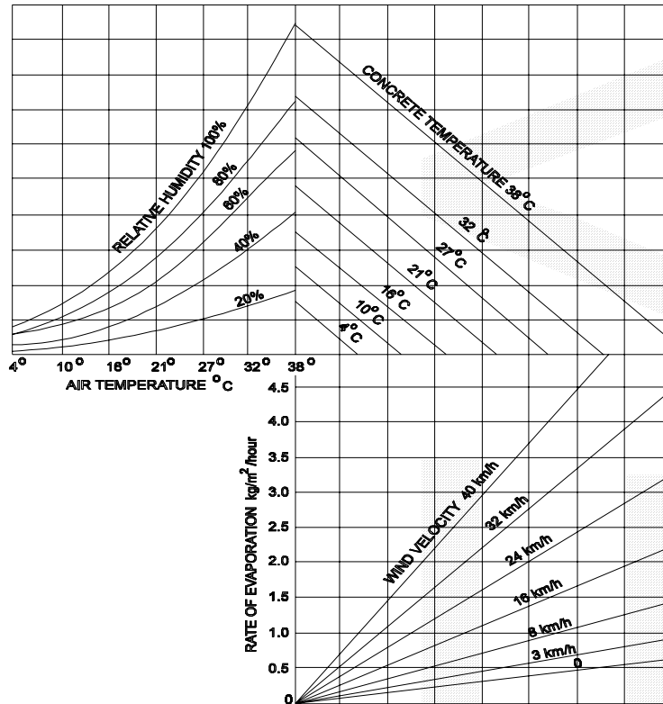
Figure C247.1 - Rate of Evaporation
